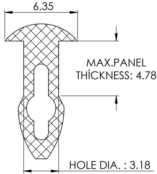
SECTION Y-Y
